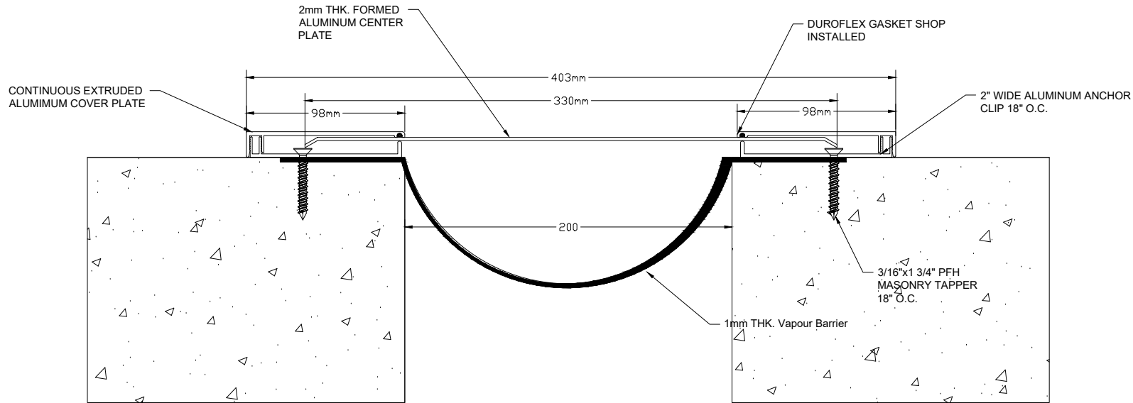
PFW-800X
