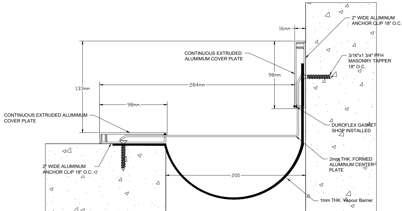
PFWC-800X
