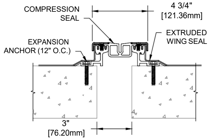
MODELS PPDA/PPDS - 300 AT OFFSET
