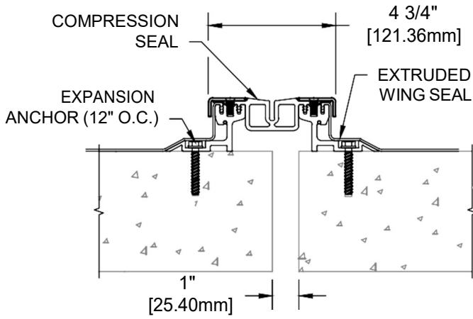
MODELS PPDA/PPDS - 100 AT OFFSET
